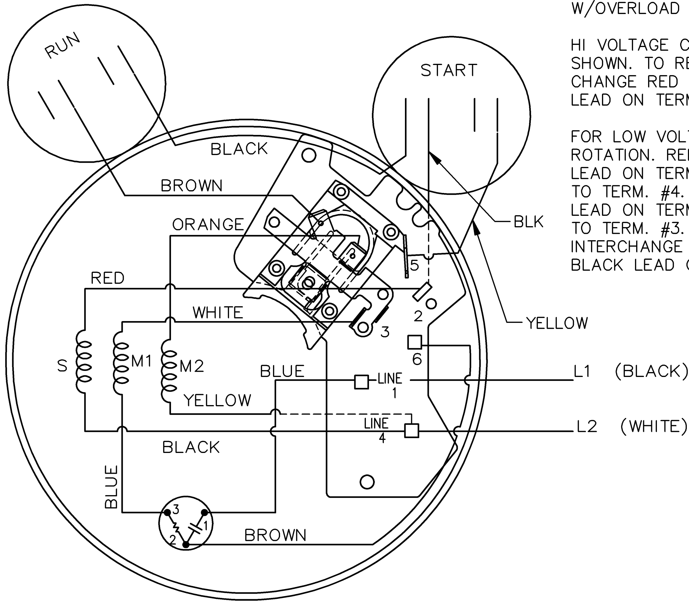
VIEW OF SHAFT END
