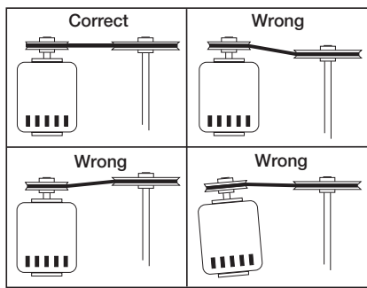
Figure 6 — Pulley Alignment
