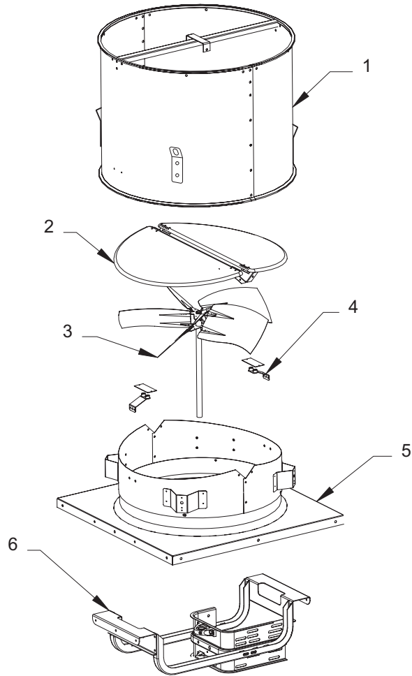
Figure 8 — Repair Parts Illustration for Axial Belt-Drive Upblast Exhaust Ventilators
