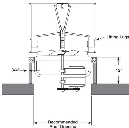
Figure 3 — Typical Roof Mounting
