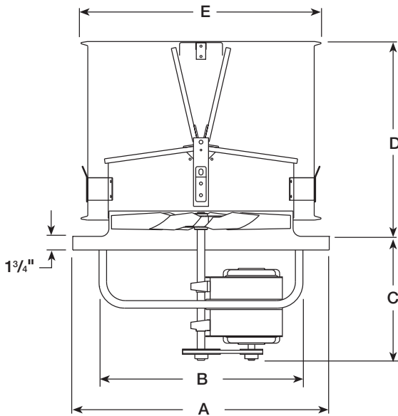
Figure 1 — Dimensions
