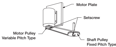
Figure 5 — Drive Package Diagram
