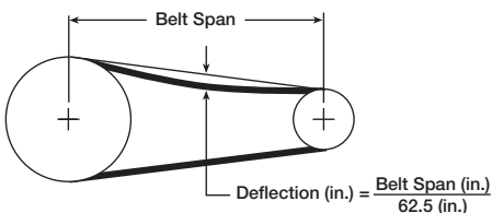
Figure 7 — Belt Tension
