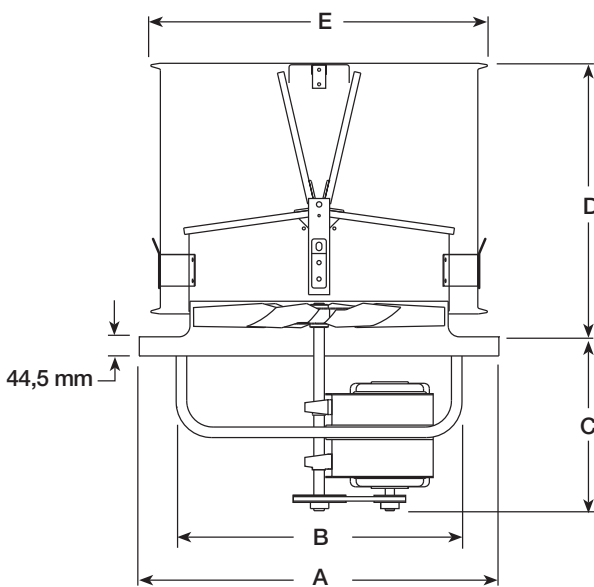
Figure 1 — Dimensions
