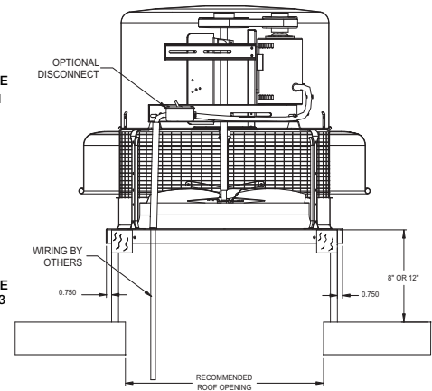
Figure 3 – Typical Roof Mounting Installation
