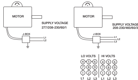
Figure 7 — Typical Wiring Diagram
