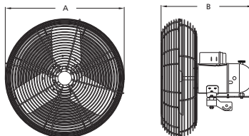
Figure 2 — Oscillating Dimensions
