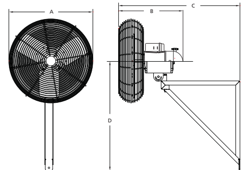
Figure 3 — 3PEG9 and 3PEH1 Dimensions
