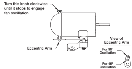
Figure 8 — Oscillating Mode
