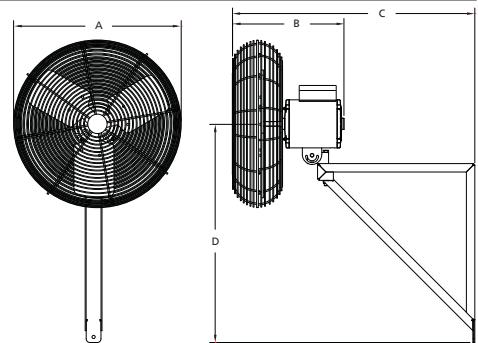
Figure 6 — 3PEH2 Dimensions
