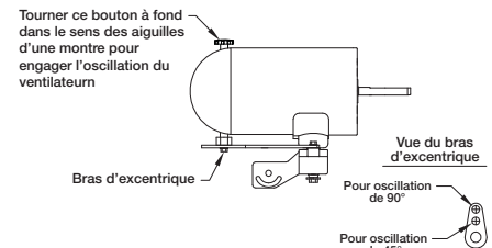
Figure 8 — Mode oscillant
