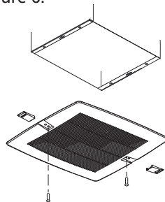
Figure 6 — Attaching Grille
