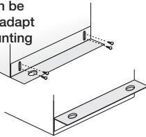
Figure 3 — Mounting Brackets
