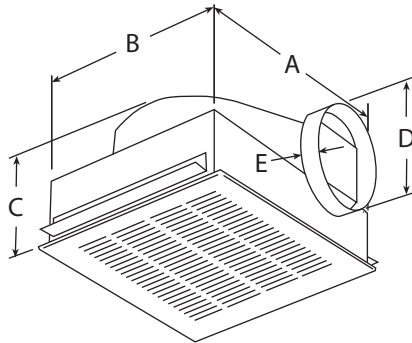
Figure 1 — Dimensions
